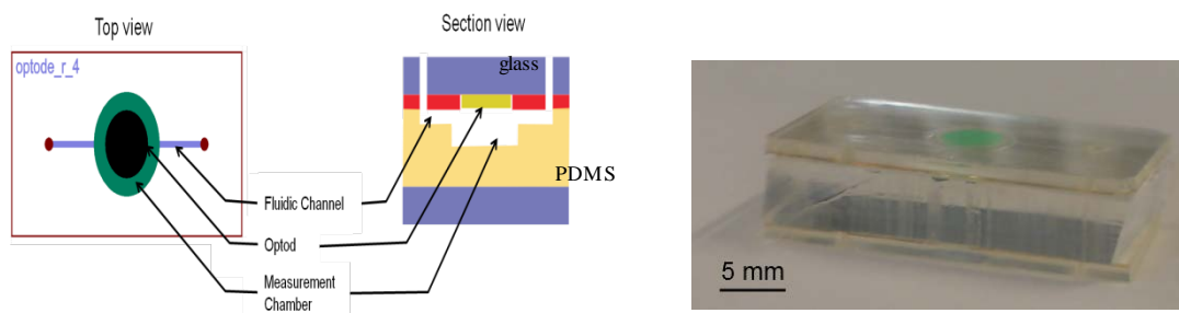
Figure 1: Schematic representation of a one-well instrumented microfluidic device and the photography of a chip ready to use. Before sealing the micro chambers, the inner walls are coated with a SU8 polymer film.
