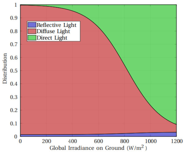
Fig. 3. The distribution of the three components of the light for a TOA irradiance of 1200 W/m 2
