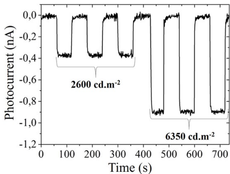
Figure S3. Evolution of photocurrent obtained for the LED luminance conditions used in this study.
