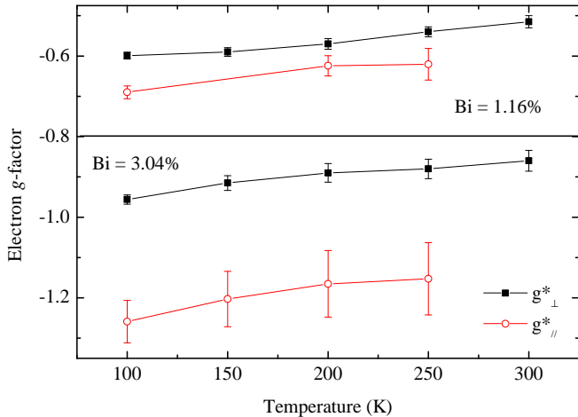
FIG. 5: Measured variation of the transverse (black closed squares) and longitudinal (red open circles) components of the electron g factor with temperature in sample 1 ( x = 1.16\% , top panel) and sample 4 ( x = 3.04\% , bottom panel) .
