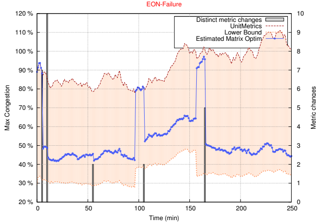
Figure 14: Congestion for EON topology with link failure
