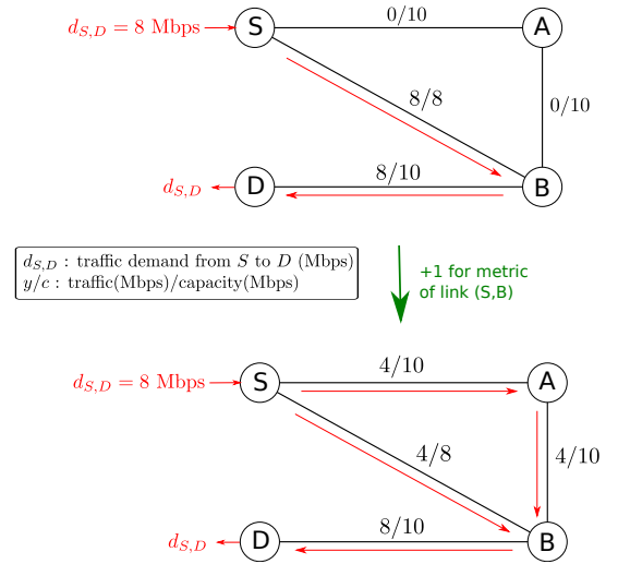
Figure 1: Metric optimization example
