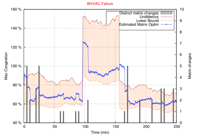
Figure 13: Congestion for BHVAC topology with link failure
