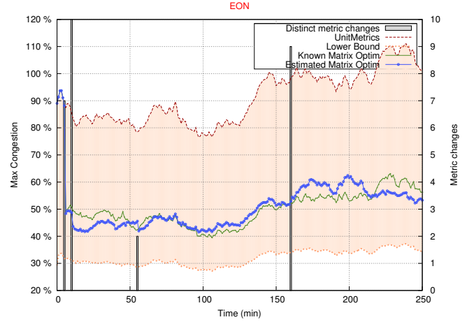
Figure 7: Congestion for EON topology
