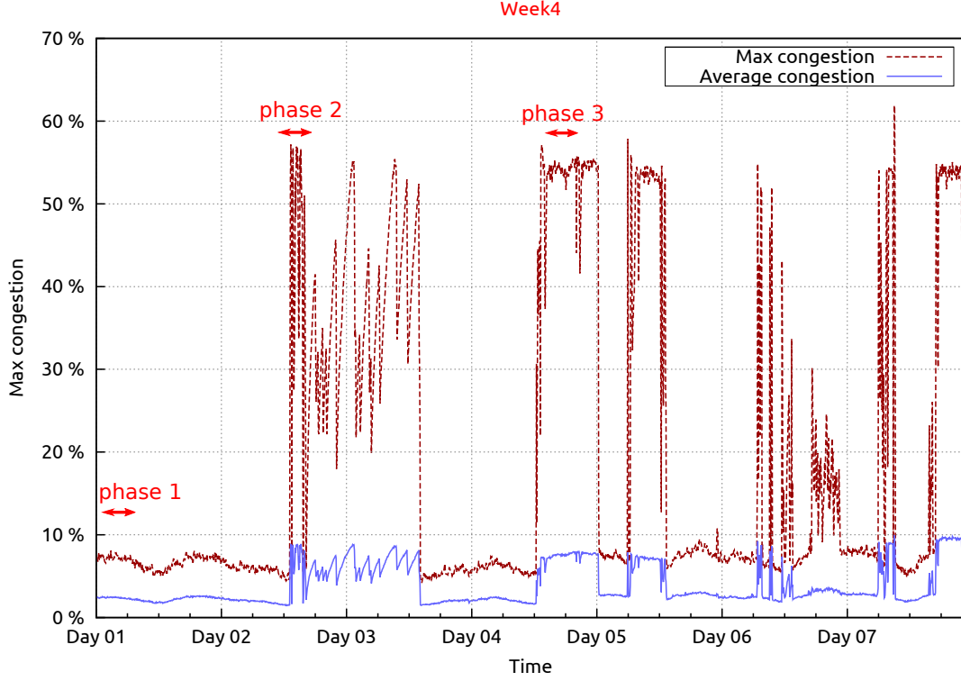
Figure 9: Link congestion rates for 4th week on ABILENE, using unit metrics
