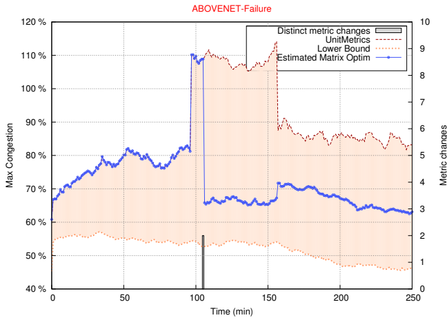
Figure 12: Congestion for ABOVENET topology with link failure
