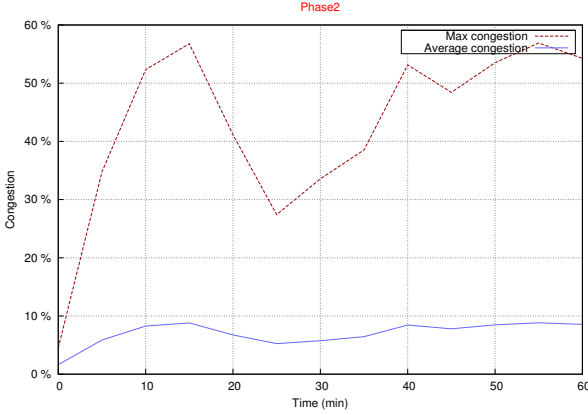
Figure 10: Zoom on phase 2
