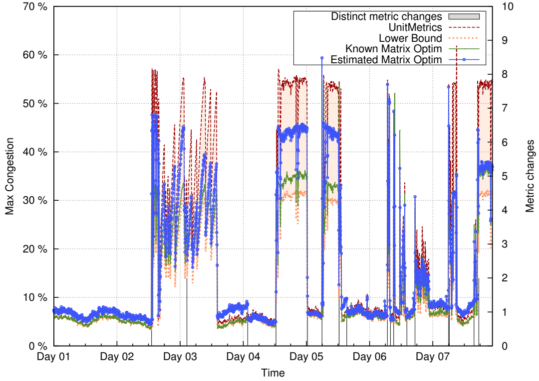
Figure 11: Congestion for ABILENE topology during the 4th week
