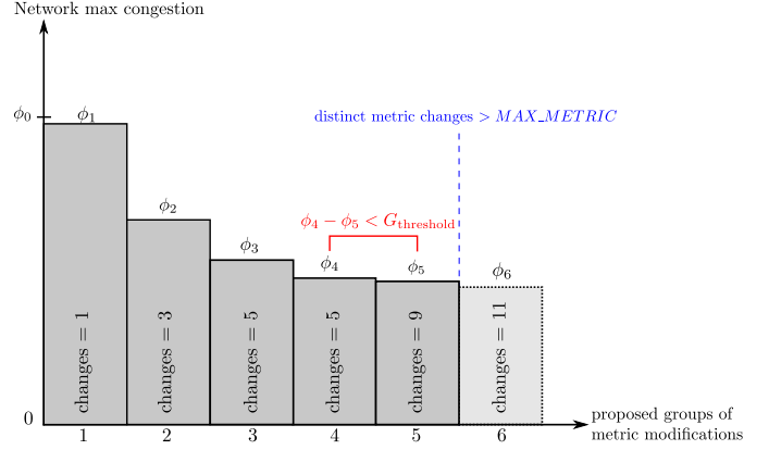
Figure 5: Restricting the number of metric changes
