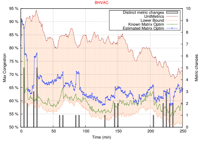
Figure 6: Congestion for BHVAC topology
