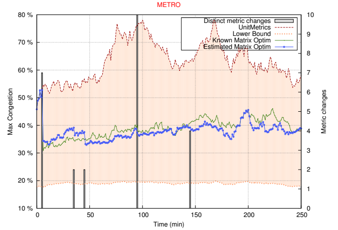
Figure 8: Congestion for METRO topology
