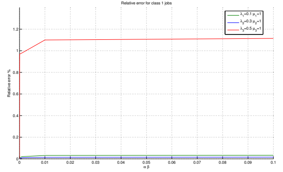
Fig. 4: Relative error for class-1 jobs.
