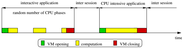
Fig. 2: Activity of an individual user across time.
