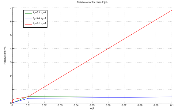
Fig. 5: Relative error for class-2 jobs.
