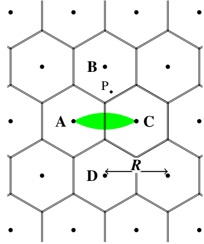
Figure 1. Topology of LoRaWAN gateways and radio coverage.
