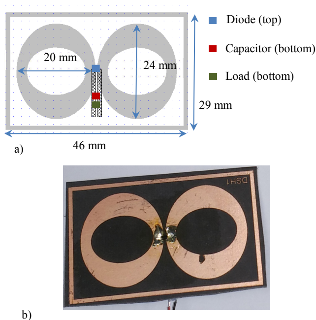
Fig. 1. Flat Dipole Rectenna (FDR): (a) the layout and the main dimensions and (b) photo of the manufactured rectenna.
