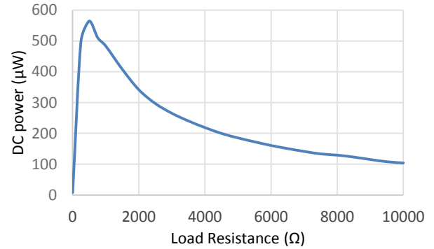
Fig.7. Measured harvested DC power as function of the load resistance for the FDR with a reflector positioned at 2.7 cm behind the rectenna (incident power density: S=33.9 \mu\text{W}/\text{cm}^2 , frequency: f=3.25 \text{ GHz} )
