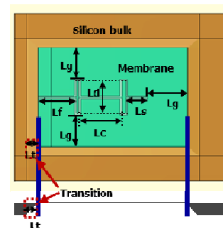
Fig. 1. Layout of the membrane supported double folded slot antenna
