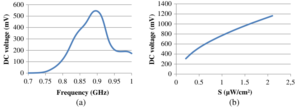
Figure 11. Measured harvested DC voltage for the manufactured rectenna (load: 10 k \Omega ) (a) as a function of frequency (b) as a function of the power density.
