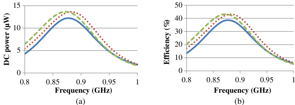
Figure 5. (a) Harvested DC power vs. frequency: HB simulation (in dotted red), co-simulation (in dashed green) and measurement (in continuous blue) results; (b) RF-to-DC conversion efficiency vs. frequency: HB simulation (in dotted red), co-simulation (in dashed green) and measurement (in continuous blue) results.
