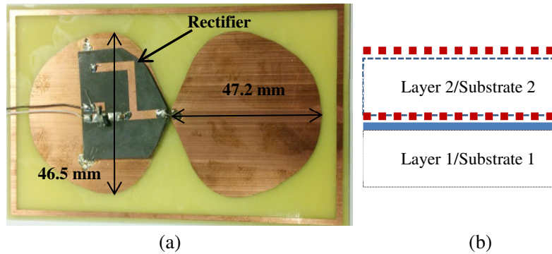
Figure 13. (a) Top view of the 2D rectenna and (b) cross sectional view of this rectenna (the continuous blue line indicates the metal layer while the dotted red lines show the metallic parts of the rectifier).
