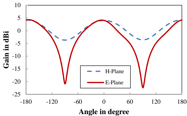
Fig. 20. Simulated (HFSS) radiation patterns in E-Plane and H-Plane at 60.2 GHz
