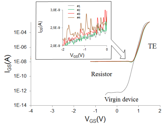
Fig. 9. Extraction of the resistive parasitic behavior from I_{GS} - V_{GS} plots in diode mode ( V_{DS}=0V ) over a batch of 5 samples (4 devices featuring a 4 \cdot 10^9 \Omega resistance, 1 virgin device feat. 10^{12} \Omega resistance), with Thermionic Emission (TE) mode used for SBH extraction.
