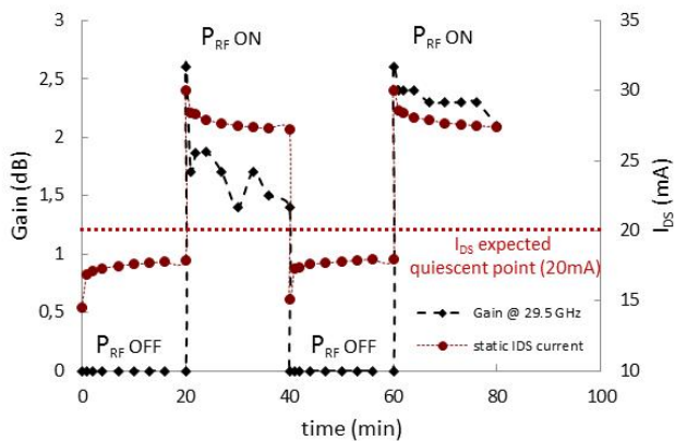
Fig. 5. Gain at 29.5 GHz and DC drain current variations versus time for a single stage LNA under non-linear CW RF signal (@ 4 dB compression point). RF signal is turned ON and OFF alternately every 20 minutes.
