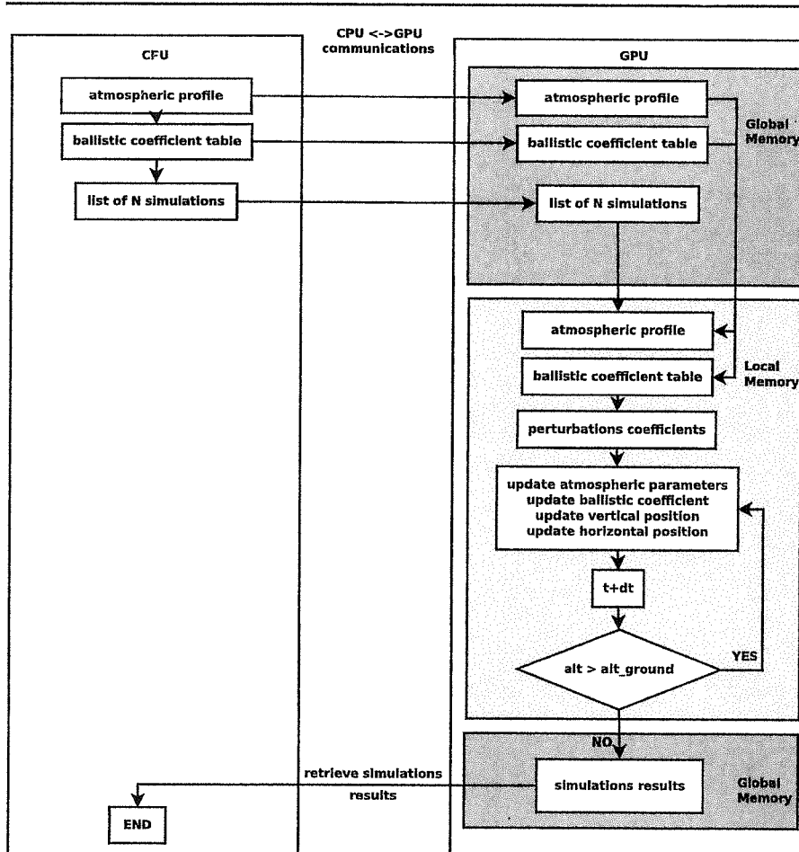
Fig. 7 GPU task parallel algorithm with memory management
