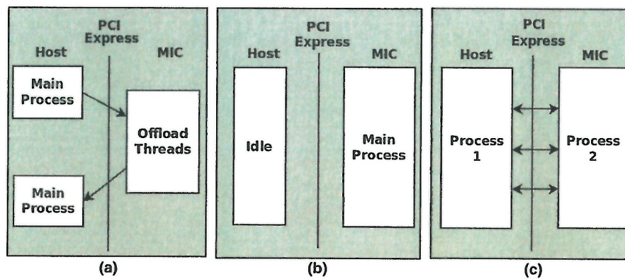
Fig. 5 Intel Xeon Phi execution modes: a offload mode, b native mode and c symmetric mode
