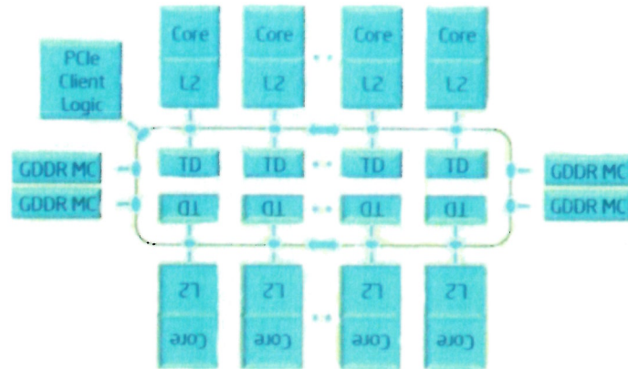
Fig. 4 Microarchitecture of the MIC coprocessor
