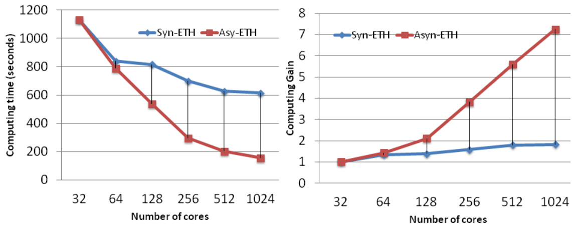
Figure 3: Computation results over Ethernet on Paravance cluster in Rennes (32 cores per computing node) in the case of the obstacle problem with size 256^3
