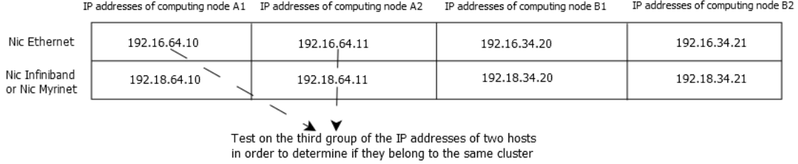
Figure 1: Example of content of Htable and test on the location of the hosts thanks to comparison of IP addresses
