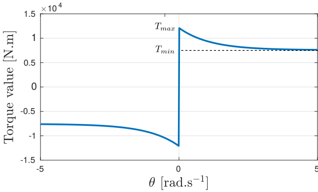
Fig. 3: Nonlinear part of the torque. T_{nl} is an approximation of the real friction torque coming from Karnopp's work [23].
