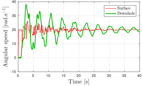
(b) System (25): \Omega_0 = 20 , \phi^0 = 0 , \phi^1 = 0 and Z(0) = 0_{2,1} .
