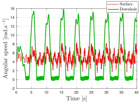
(c) System (25): \Omega_0 = \phi^1 = 5 , \phi^0(x) = (1 + 0.1 \sin(x)) \int_0^x \phi_x^\infty(s) ds and Z(0) = (z_1^\infty \ z_2^\infty)^\top .
