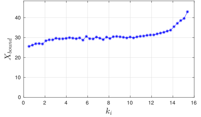
(a) X_{bound} for k_p = 10^{-3} but with different values of k_i
