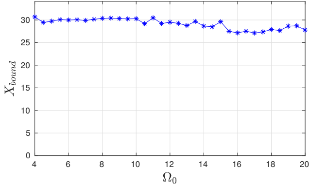
Fig. 9: Solution X_{bound} of BMI (27) for k_p = 10^{-3} , k_i = 10 , \tau_0 = 0.0153 and N = 5 .
