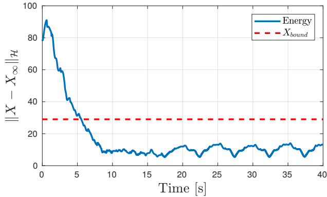
Fig. 10: Energy of X with the nonlinear system for k_p = 10^{-3} , k_i = 10 and \Omega_0 = 5 . The initial condition is the same than in Figure 5.
