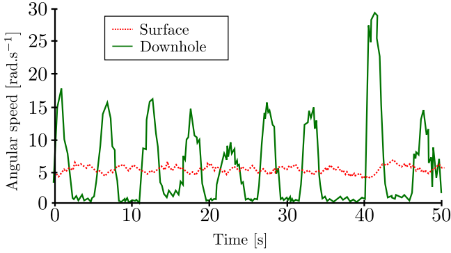
Fig. 2: Nonlinear effect on the drilling mechanism due to the friction torque at the bottom of the pipe. These measurements are done on the field [41].
