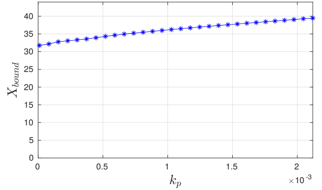
(b) X_{bound} for k_i = 10 but with different values of k_p
