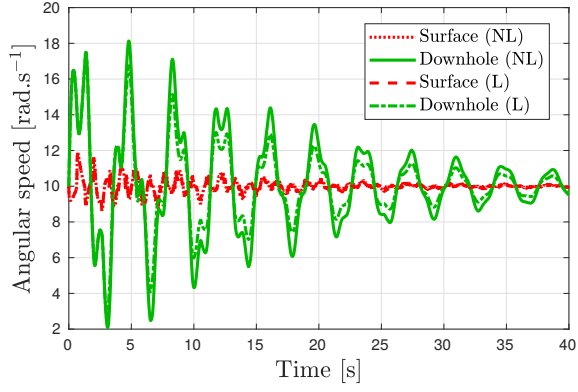
(a) Systems (10) and (25): \Omega_0 = \phi^1 = 10 , \phi^0(x) = (1 + 0.32 \sin(x)) \int_0^x \phi_x^\infty(s) ds and Z(0) = (z_1^\infty \ z_2^\infty)^\top .
