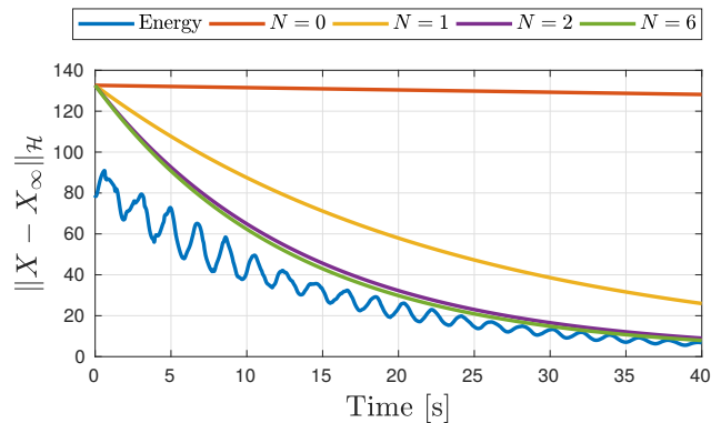
Fig. 5: Energy of X with the linear system for k_p = 10^{-3} , k_i = 10 and \Omega_0 = 5 . The initial condition is \phi^0(x) = 4 (\int_0^x \phi_x^\infty(s) ds + 0.1 \cos(2x)) , \phi^1 = 2\Omega_0 and Z(0) = 2 [z_1^\infty \ z_2^\infty]^\top .
