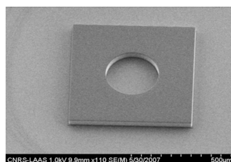
Figure 8: Picture BPR 100- micro-cavity.
