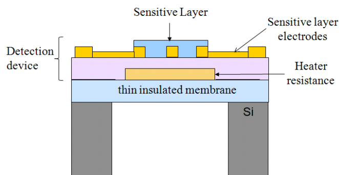
Figure 1: Structure of gas sensor.
