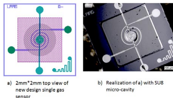
Figure 6: Single gas sensor with SU8 micro-cavity.
