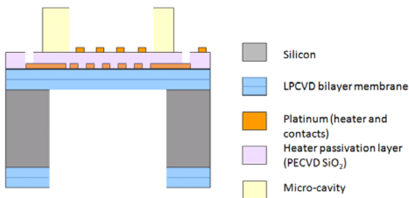
Figure 9: Structure of new gas sensor.
