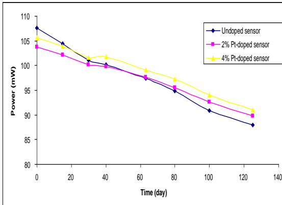
Figure 2: Time drift for 3 gas sensors.
