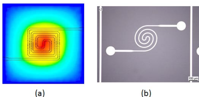
Figure 5: Different designs of micro-hotplate.
