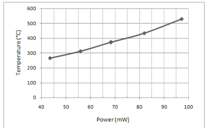
Figure 10: Temperature reached versus power.
