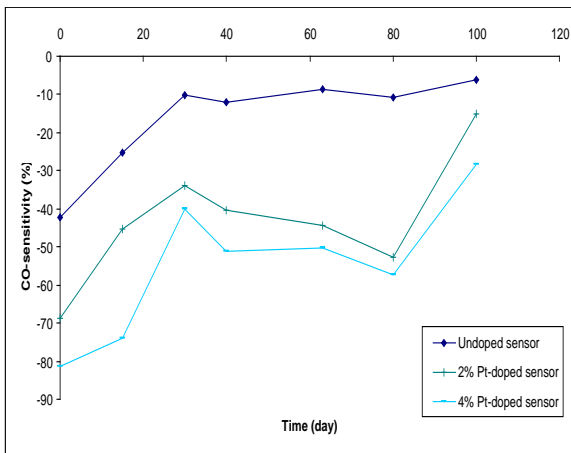
Figure 3: CO-sensitivity versus time (100 days) for the previous gas sensors.
