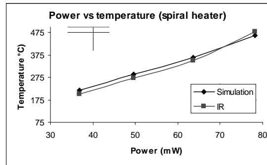
Figure 4: Temperature reach versus power.
