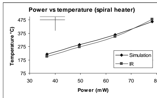
Figure 4: Temperature reach versus power.
