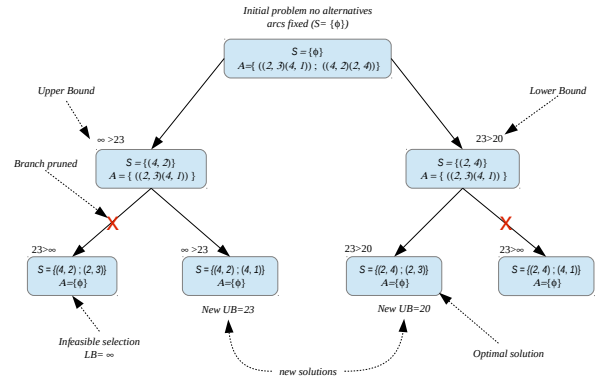
Figure 6. Search tree for the BJSS instance.
