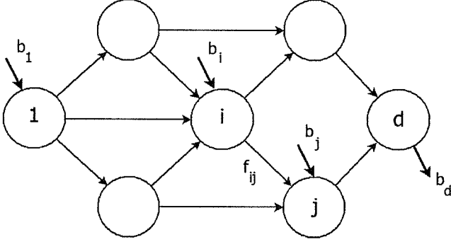
Fig. 1. Single destination network flow
