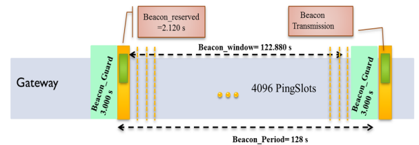
Fig. 5: class B - Beacon Timing
