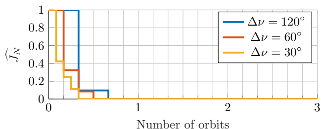
Fig. 4: Normalized cost for N = 3 over the first 3 periods
