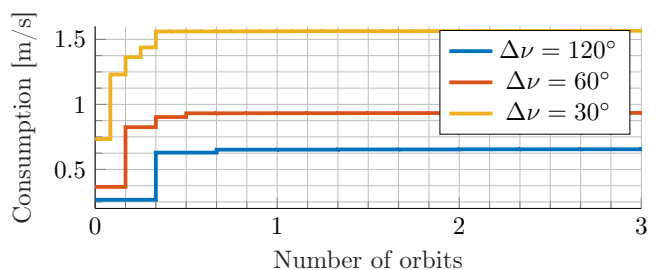
Fig. 3: Consumption for N = 3 over the first 3 periods
