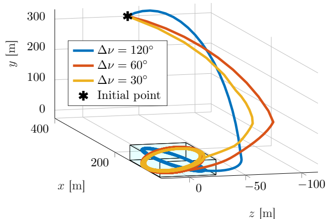
Fig. 2: Relative trajectories from X_{01} with N = 3 and different \Delta\nu
