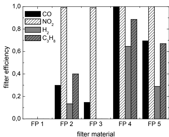
Figure 3. Filter efficiency for the five tested filter materials and the four test gases allowing fast assessment of the filter performance.
