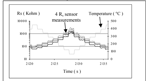
Fig. 6: Profile of operating temperature.
