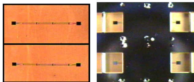
Figure 3 : Two bandpass filters shown before and after shielding
