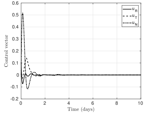
Figure 4: Control profile.
