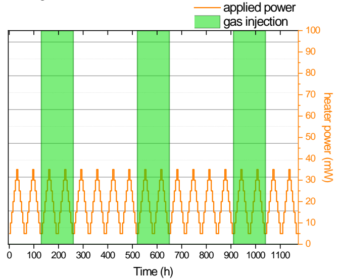
FIGURE 3: Test protocol for the micro-sensors.
