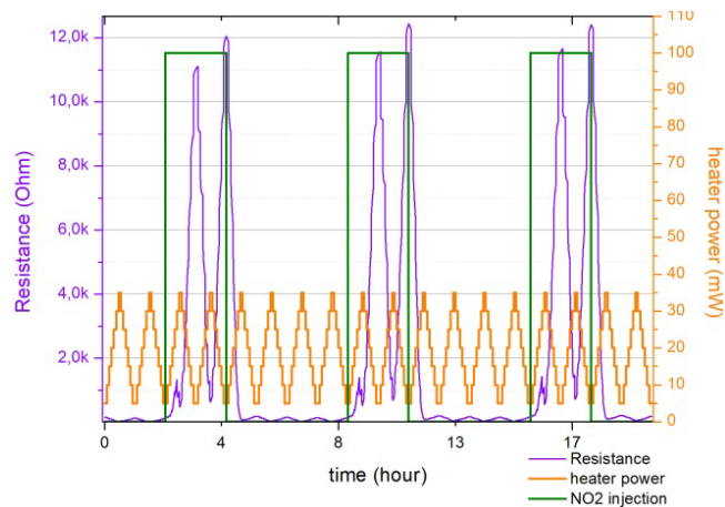
FIGURE 7: Evolution of the resistance of 50 nm thick ZnO:Ga layer under air and air + 500 ppb of \text{NO}_2 (with 50% relative humidity).
