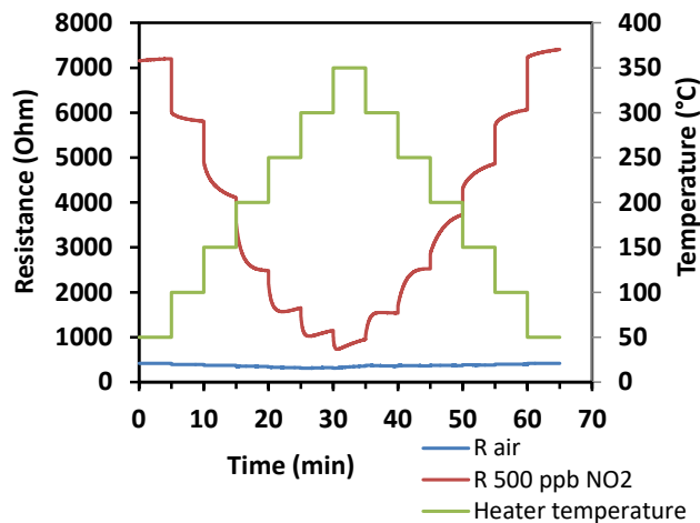
FIGURE 8: Resistance variation under Air (in black) and under \text{NO}_2 (in red).
