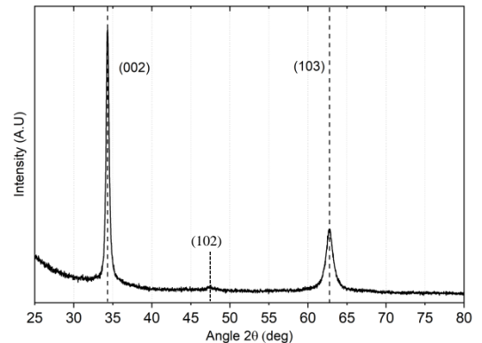
FIGURE 4: XRD pattern of 50 nm thick \text{ZnO:Ga} thin film.
