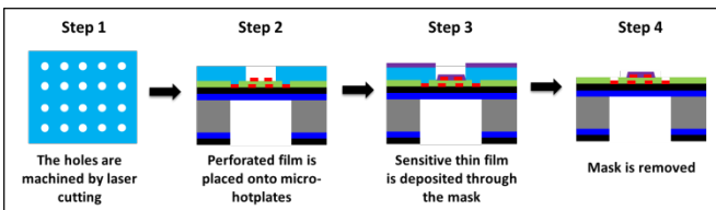
FIGURE 2: Integration process of \text{ZnO:Ga} using stencil mask.
