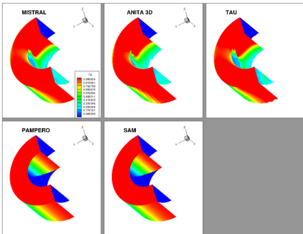
Figure 7: pressure coefficient for case M002: hollow cylinder at 45° AoA
