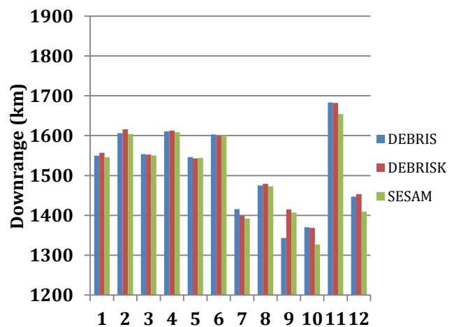
Figure 19: Downrange in km of the Integration cases
