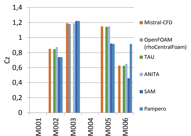
Figure 6: Normal force coefficient for Mandatory Cases
