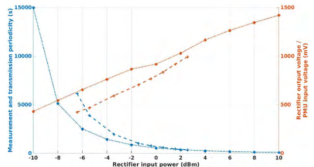
FIGURE 7. Measurement and transmission periodicity (blue) and rectifier output voltage (orange) in function of the applied RF input power for the prototype supplied by a controlled RF power at the input of the rectifier (*), by a controlled power density illuminating the rectenna in an anechoic chamber (+). In this case, the RF power at the input of the rectifier is estimated by taking into account the simulated gain of the antenna integrated into the rectenna.
