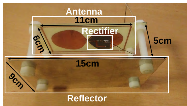
FIGURE 3. Photograph of the manufactured rectenna.
