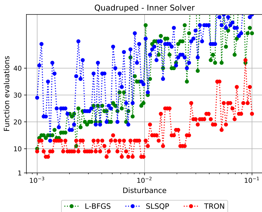
FIGURE 3.8: Quadruped inverse geometry problem, evaluation of inner solvers in augmented Lagrangian. Optimization starts from the optimal values of a reference problem (warmstart). The problem variation with respect to the reference is parameterized by the disturbance.
