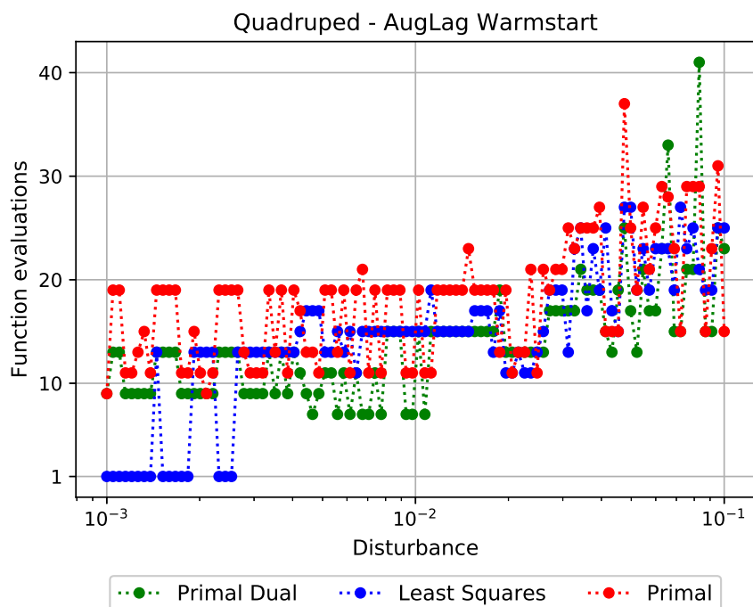
FIGURE 3.10: Quadruped inverse geometry problem, evaluation of different warmstart strategies for the augmented Lagrangian. The problem variation with respect to the reference is parameterized by the disturbance.
