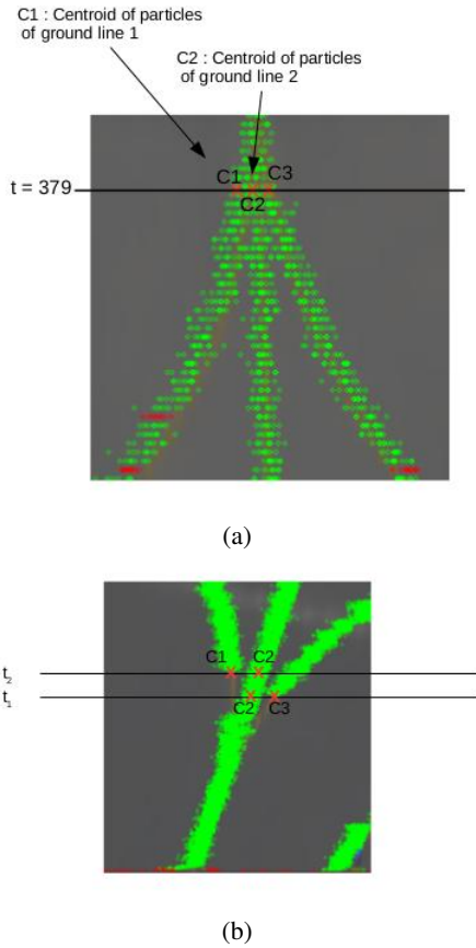
Figure 10: (a) Fusion of clusters, (b) New lane tracking
