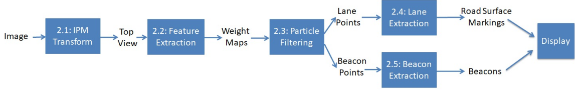
Figure 1: Functions for interpretation of airport scenes
