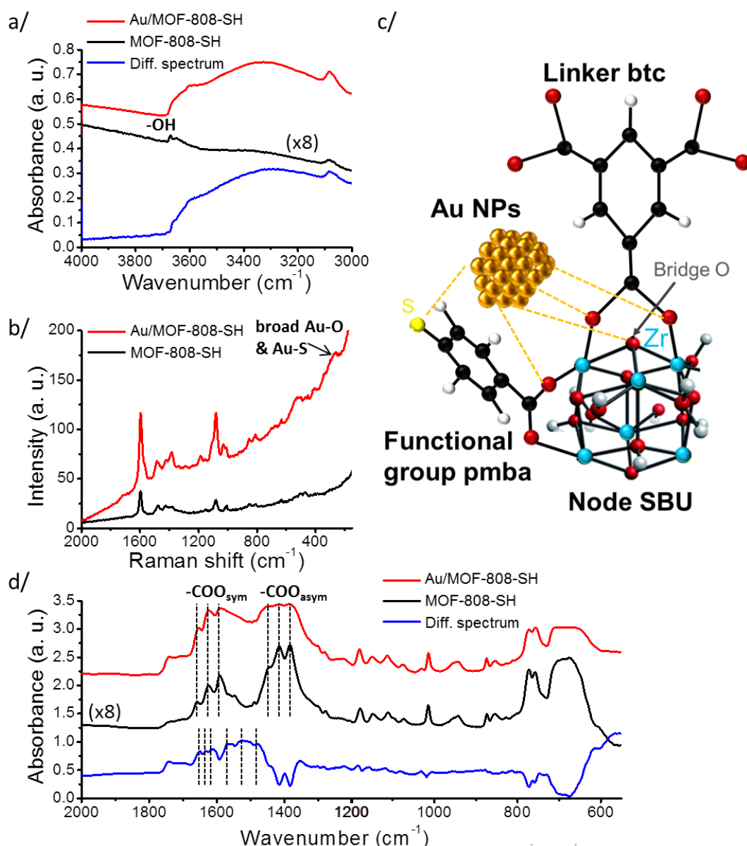
Figure 5. (a) Infrared spectra of the 4000–3000 \text{cm}^{-1} region; (b) Raman spectra; (c) schematic representation of the interactions between Au NPs and MOF-808-SH; (d) infrared spectra of the 2000–550 \text{cm}^{-1} region for Au/MOF-808-SH (red curves) and MOF-808-SH materials (black curves). Differential spectra are depicted as blue.
