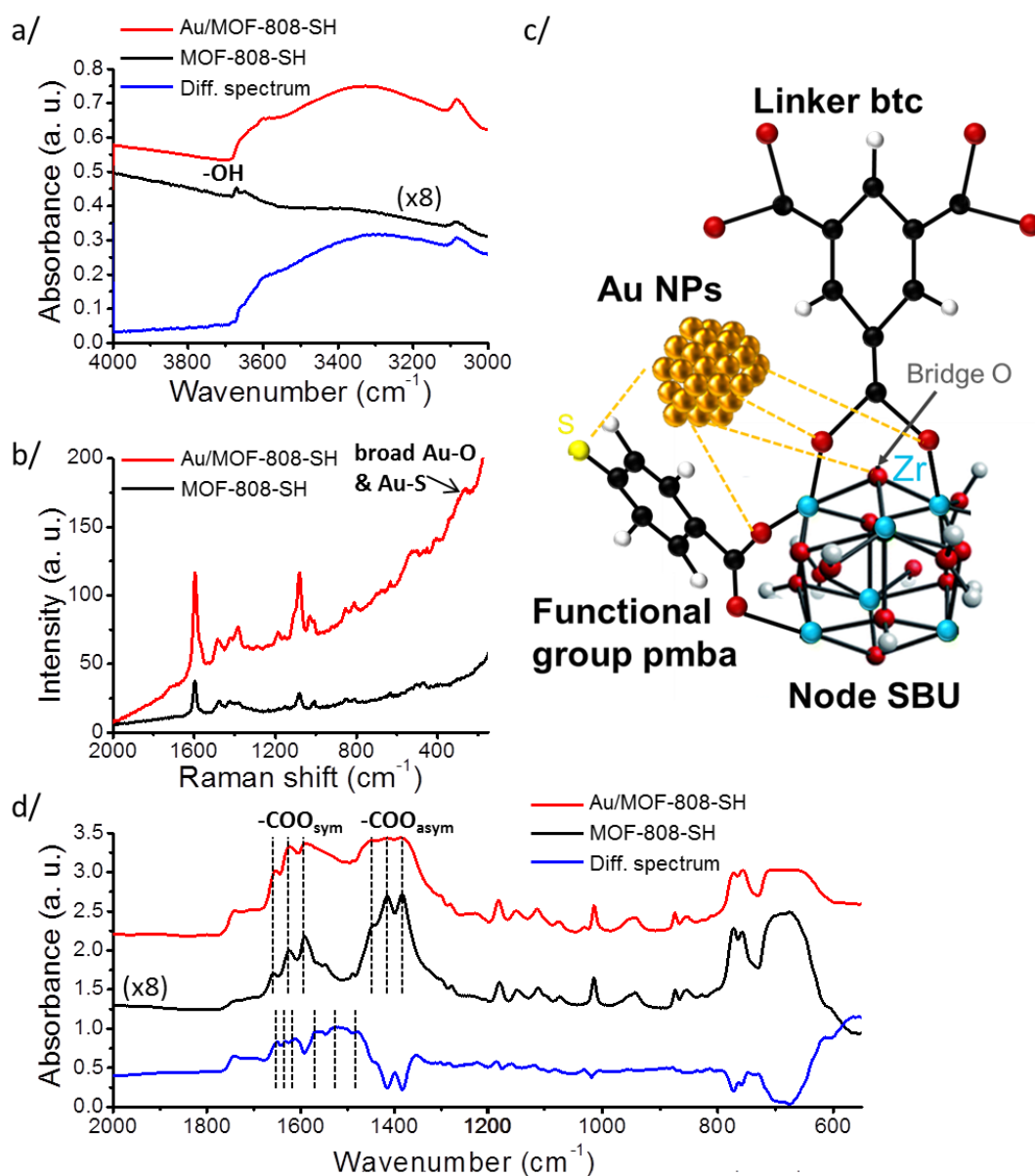
Figure 5. (a) Infrared spectra of the 4000–3000 \text{cm}^{-1} region; (b) Raman spectra; (c) schematic representation of the interactions between Au NPs and MOF-808-SH; (d) infrared spectra of the 2000–550 \text{cm}^{-1} region for Au/MOF-808-SH (red curves) and MOF-808-SH materials (black curves). Differential spectra are depicted as blue.
