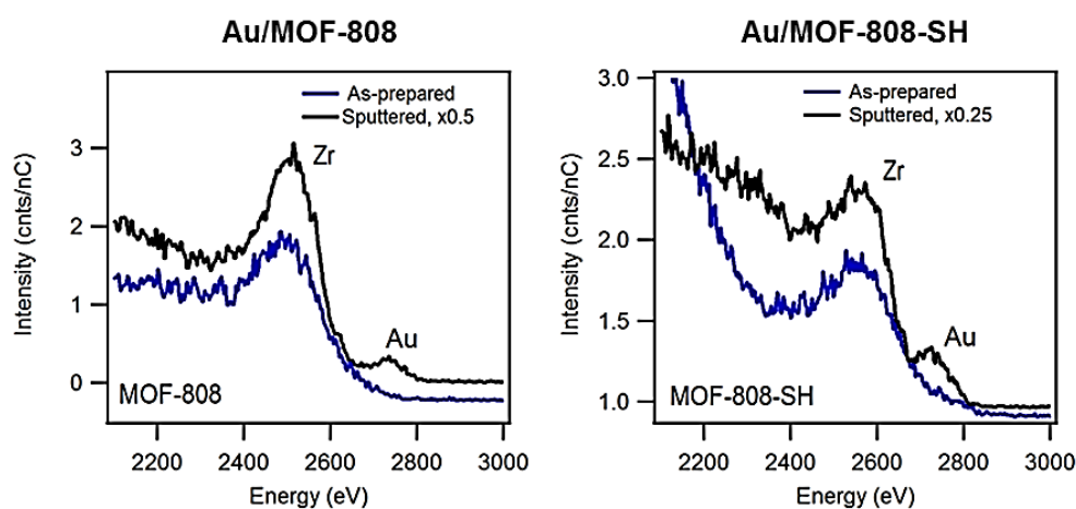
Figure 3. LEIS spectra of Au/MOF-808 and Au/MOF-808-SH before (blue) and after (black) sputtering ( 4 \times 10^{14} \text{ cm}^{-2} \text{ Ar}^+ ), using 3 \text{ keV He}^+ ions. Spectra corresponding to the sputtered sample are scaled for ease of comparison to the spectra of the as-prepared material.
