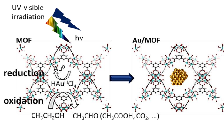
Figure 1. MOFs as nano-reactors for the growth of Au NPs via photo-reduction.
