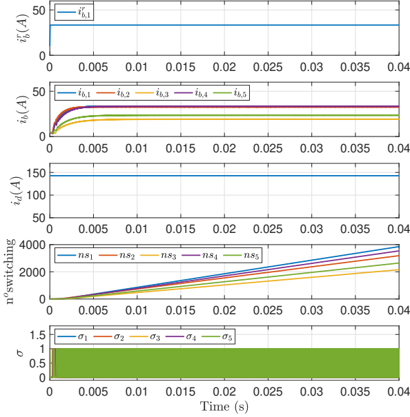
Fig. 7: From the top, the following evolutions: current reference of the leader \mathcal{N}_1 , i_{b,i}^r , output currents of each node, i_b , demanded current i_d , number of switching of each node and discrete input variables \sigma_i , when connection \mathcal{E}_3 fails at 0.01s and \mathcal{E}_1 fails at 0.025s.
