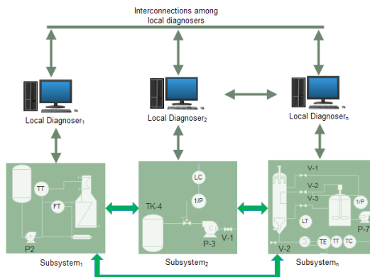
Fig. 2. Distributed diagnosis architecture
