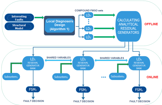
Fig. 3. Scheme of distributed generation of LDs.
