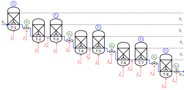
Fig. 1. Diagram of the flotation process under study.
