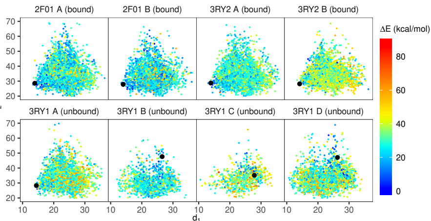
Fig. S11. 2D projections of conformations sampled using RCD+ for a loop in the streptavidin protein, from eight starting X-ray crystallography protein structures. The first dimension, d_1 (x-axis), is the distance (Å) between an atom located in the middle of the loop and a fixed atom in the protein. The second dimension, d_2 (y-axis), is the angle (degrees) formed by three atoms: an atom at approximately one quarter, one half, and three quarters of the way down of the loop. The conformations from the crystallographic structures are shown in black. For each system, the loop with the lowest energy was identified and each conformation was then colored according to the difference between its energy and this lowest energy.
