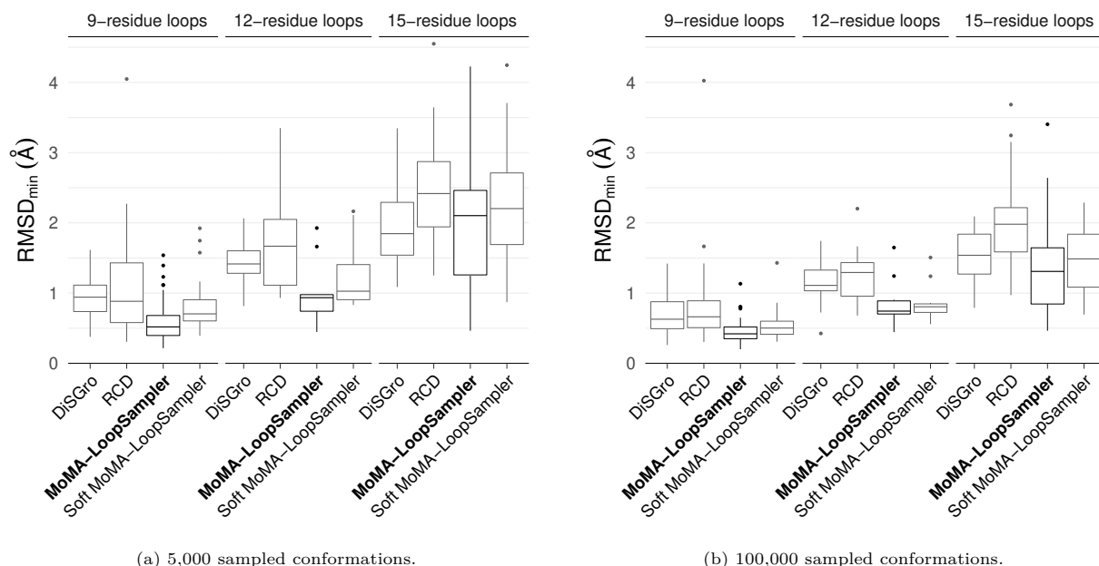
Fig. S7. Minimum distance to native ( \text{RMSD}_{\min} ) obtained among sampled conformations, without side-chains.
