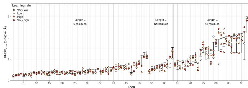
Fig. 4. RMSD_{min} of MoMA-LoopSampler on each loop ensemble. Diamonds correspond to the results obtained for each learning rate. Error bars show the RMSD_{min} range obtained by the four tests performed without H_{RL} . A data point above the error bar shows that the corresponding run with H_{RL} misses some closer-to-native conformations that can be sampled when turning H_{RL} off. A data point below the error bar indicates that the corresponding run found conformations that are even closer to native than the runs without learning did.
