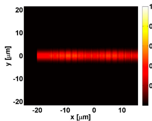
Fig. 6 Self-normalised Poynting vector at 1567 nm (linear scale), considering the value of the source waist radius w_0 = 15a/2
