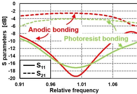
Fig. 7. Measured S-parameters at the atmospheric pressure as a function of the ratio f/f_{res} (where f_{res}=23\text{GHz} and f denotes the frequency) achieved for two assembling processes: photoresist bonding (in green) and anodic bonding (in red).
