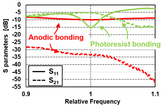
Fig. 14. Measured S-parameters at the atmospheric pressure as a function of the ratio f/f_{res} (where f_{res}=23\text{GHz} and f denotes the frequency) achieved for the sensors assembled from two manufacturing processes: photoresist bonding (in green) and anodic bonding (in red) assembling processes.
