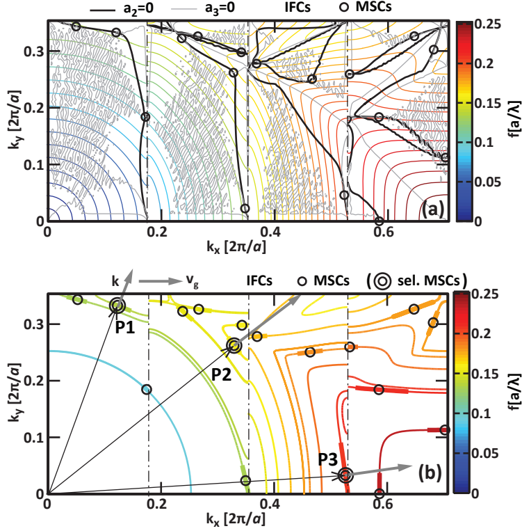
Fig. 3. (a) zero a_2 (black curves) and zero a_3 (gray thin curves) loci for the F_4 MPhC. Black circles highlight the crossing points where non-trivial MSC is ensured. (b) IFCs corresponding to the solutions found.
