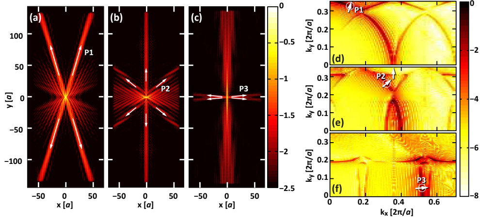
Fig. 4. (a) (b) (c) Logarithm of the self-normalised Poynting vector magnitude when a F_4 MPhC structure is excited by a point source placed in its center, at the reduced frequencies of the solutions : (a) P1 0.1367[a/\lambda] (b) P2 0.1607[a/\lambda] and (c) P3 0.2043[a/\lambda] . (d) (e) (f) Corresponding logarithm of the self-normalised magnitude of the spatially Fourier transformed z -component of the magnetic field.
