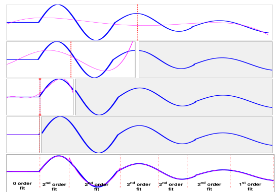
Figure 1. Interval halving polynomial approximation
