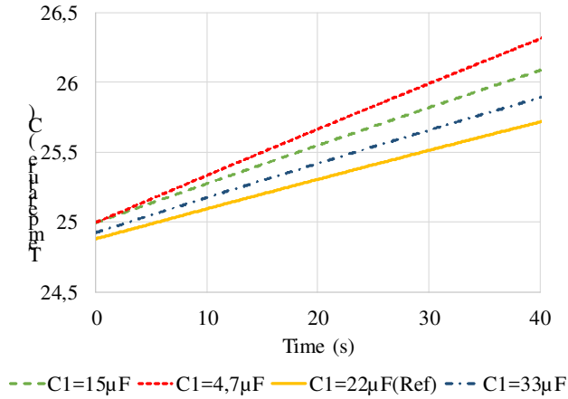
Fig. 10. IRTS measured over C1 for three defect values in comparison with the reference IRTS.
