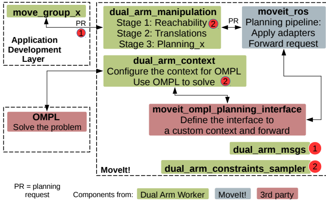
Fig. 5: Functional view of the developed packages to solve a dual-arm planning request. The numbers 1, 2 indicate where the two unconnected components at the bottom are used.
