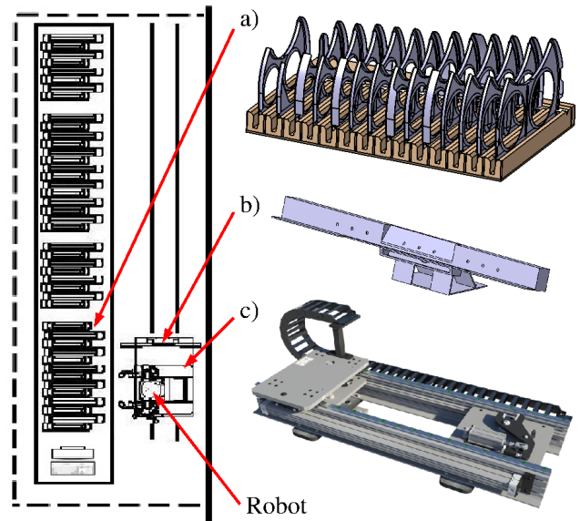
Fig. 2: Lay-out and main elements of the work-cell: a) rib container rack; b) deburring support; c) lineal track.
