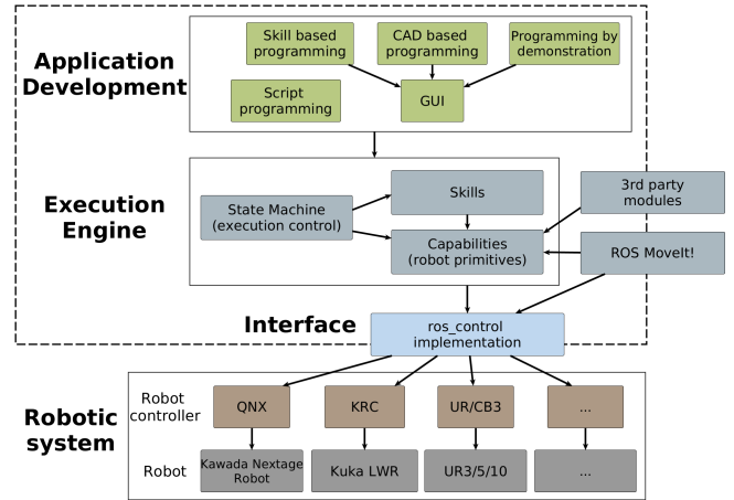
Fig. 3: Three-layer-based software architecture: application development through diverse approaches, execution engine for task execution and capability management, and interface with the actual robotic systems.
