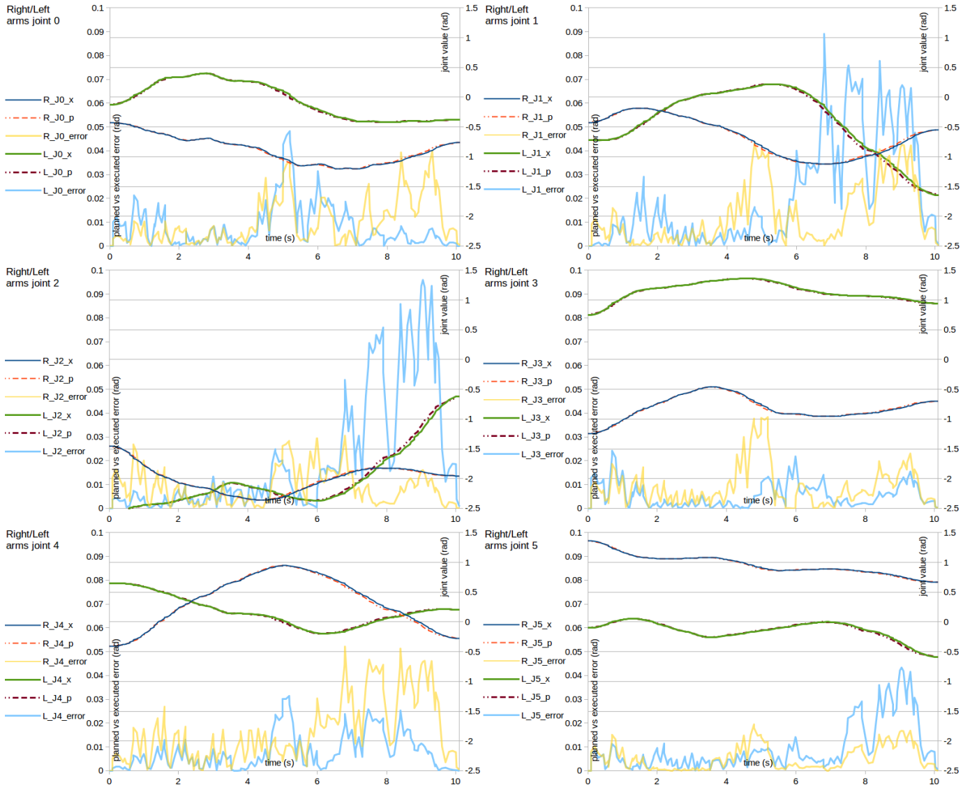
Fig. 6: Comparison of the right and left arms joint values for motion Md_4 between a planned trajectory and the executed one.
