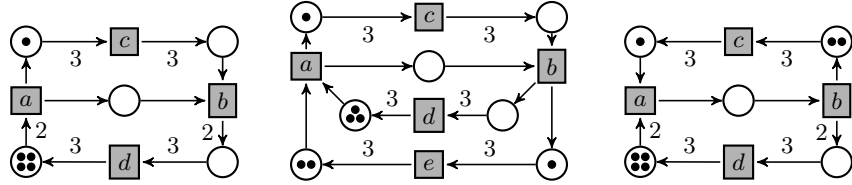
Fig. 4. The WMG on the left solves aacbdbl cyclically, and the WMG in the middle solves aacbbed cyclically. On the right, the WMG solves abcabd cyclically.
