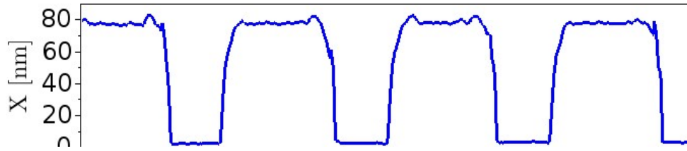
Fig. 4. Atomic-Force Microscope measurement of the profile of the etched grating into the SiN layer.
