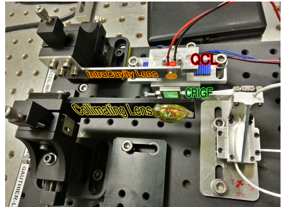
Figure 4. Extended cavity quantum cascade laser.
