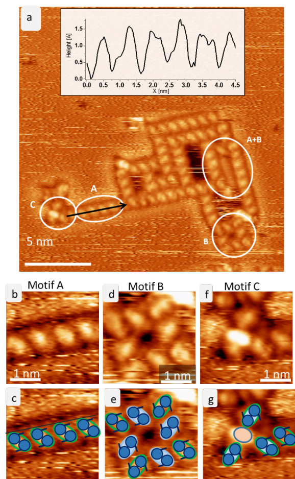
Figure 2: The three ordered motifs A-C of trehalose on Cu(100). a) STM image showing the assembly of trehalose on Cu(100) at room temperature. The three different motifs A-C are marked. A line profile is shown in the inset. b) Magnification of motif A depicting a line of skewed molecules. c) A sketch of motif A. The green lobes correspond to single trehalose molecules, the two blue circles indicate the two saccharide subunits. d) Zoom into motif B depicting the squared arrangement of 8 trehalose molecules. e) Sketch of motif B. f) Zoom into motif C. g) Sketch of motif C.
