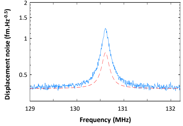
Figure 4: (Blue) Brownian motion of the optomechanical resonator measured at 1-Hz bandwidth. Resonance frequency is f_m=130.6 MHz. The sensor’s quality factor attains Q_m=1000 in air. The signal is calibrated via detection chain. (Red) Brownian motion theory given by the equipartition theorem with same noise floor. The 1.7 factor between theoretical and measured noise amplitude is within detection parameters uncertainty.
